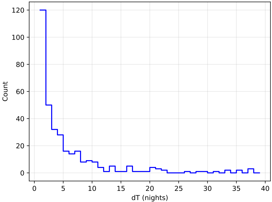
roll_pause_mjdp0_v3.4_10yrs all bands: DD:WFD Delta Nights Histogram
