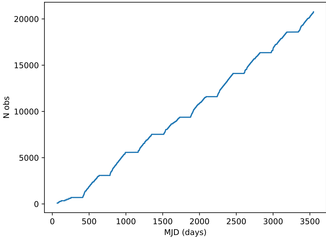
roll_pause_mjdp0_v3.4_10yrs all bands: DD:ELAISS1 Cumulative NVisits
