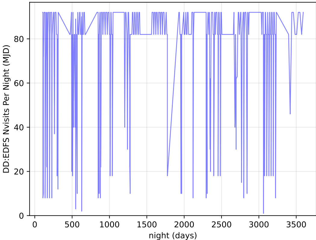
roll_pause_mjdp0_v3.4_10yrs all bands: DD:EDFS Nvisits Per Night
