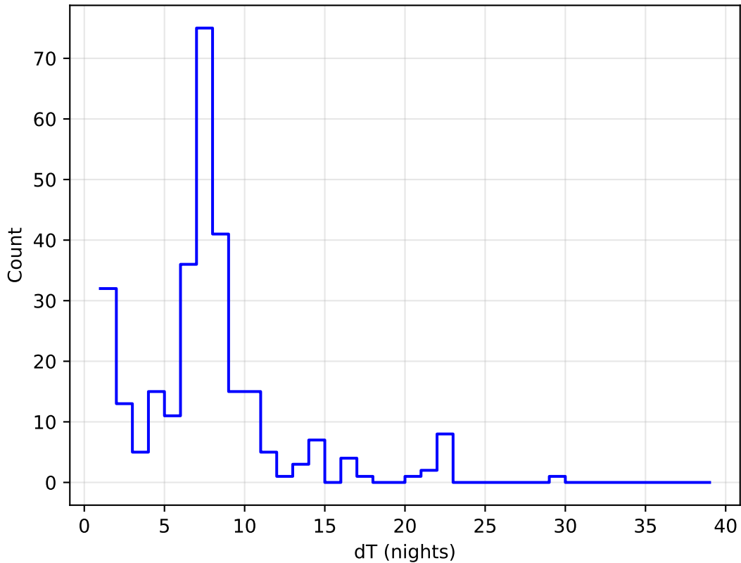
roll_pause_mjdp0_v3.4_10yrs all bands: DD:EDFS Delta Nights Histogram
