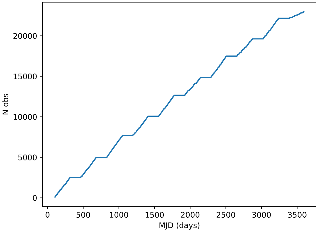
roll_pause_mjdp0_v3.4_10yrs all bands: DD:EDFS Cumulative NVisits
