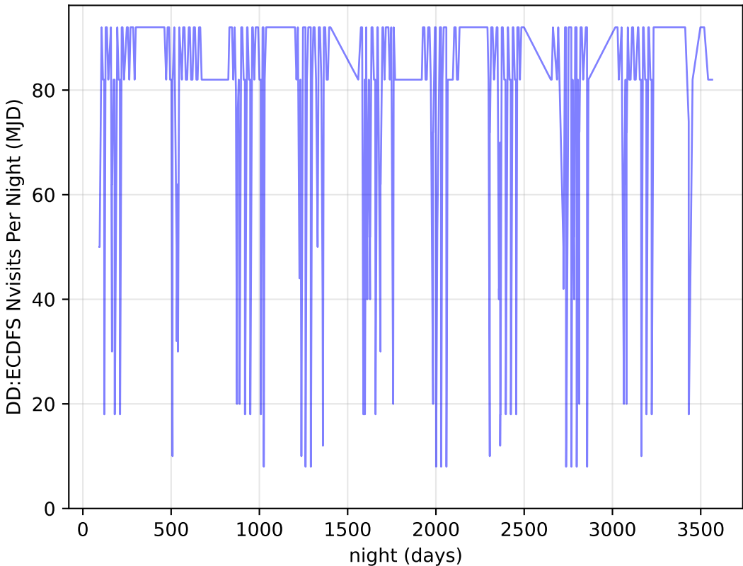
roll_pause_mjdp0_v3.4_10yrs all bands: DD:ECDFS Nvisits Per Night
