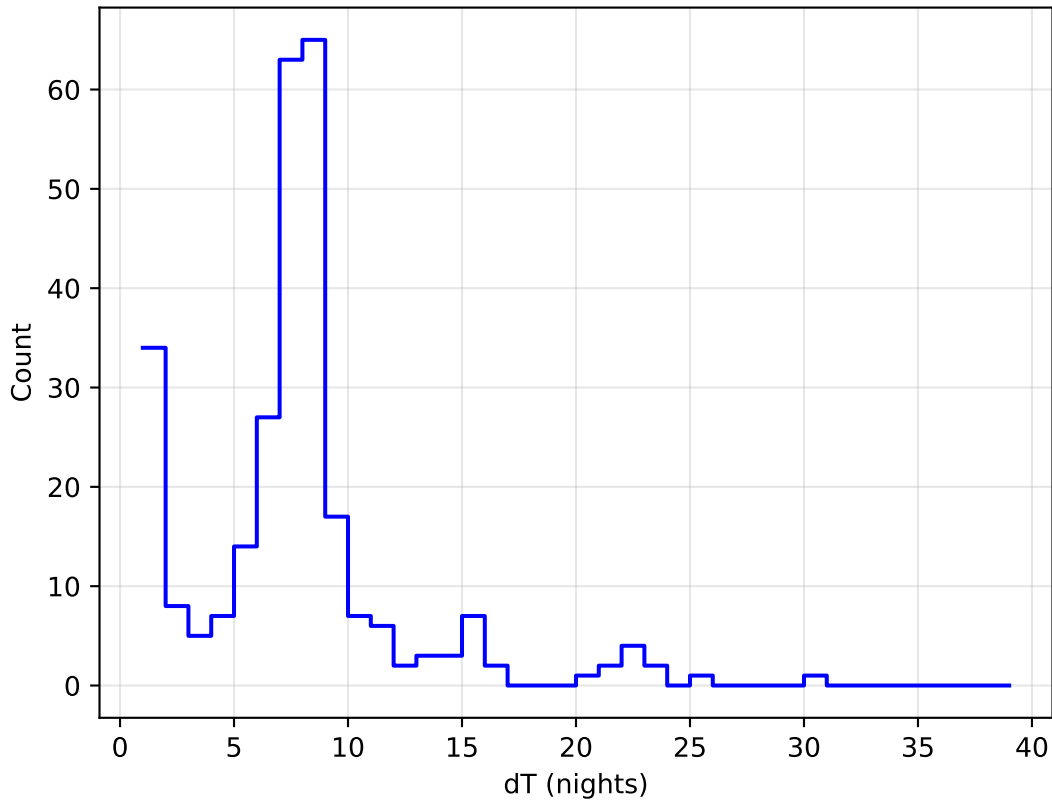
roll_pause_mjdp0_v3.4_10yrs all bands: DD:ECDFS Delta Nights Histogram
