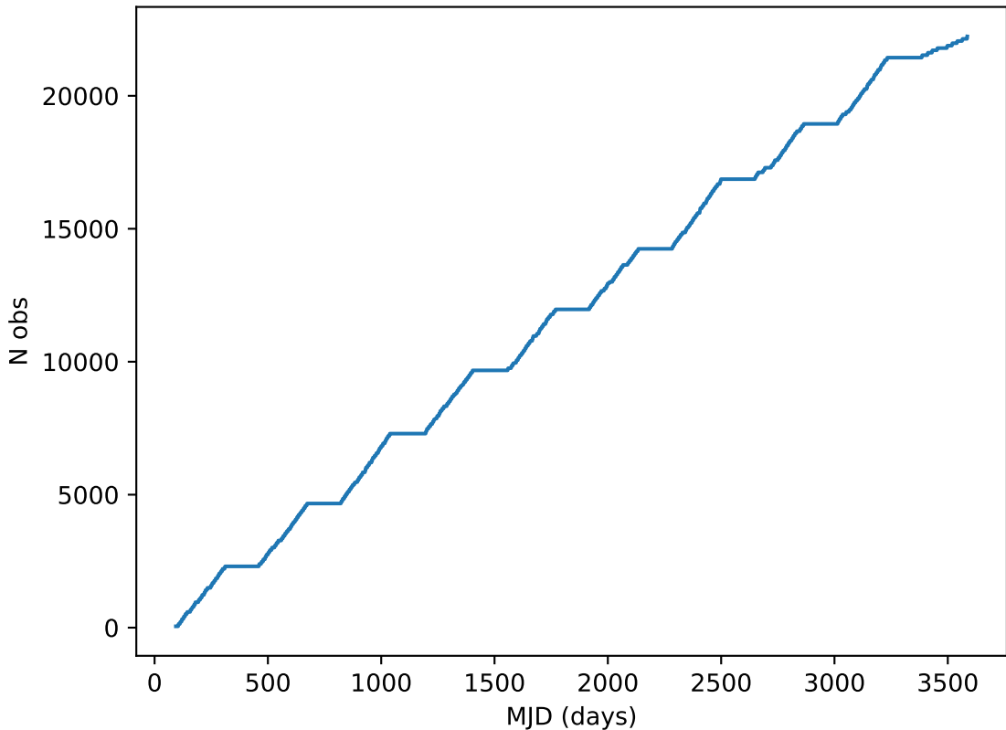
roll_pause_mjdp0_v3.4_10yrs all bands: DD:ECDFS Cumulative NVisits
