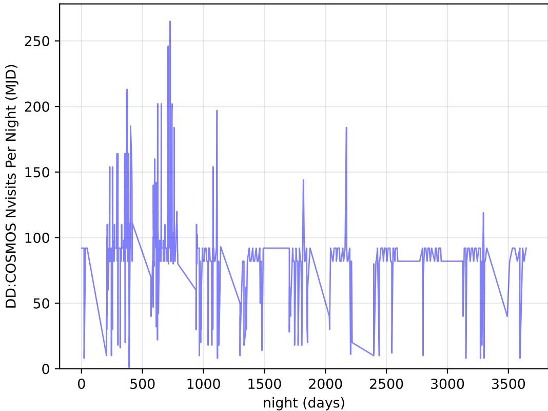
roll_pause_mjdp0_v3.4_10yrs all bands: DD: COSMOS Nvisits Per Night
