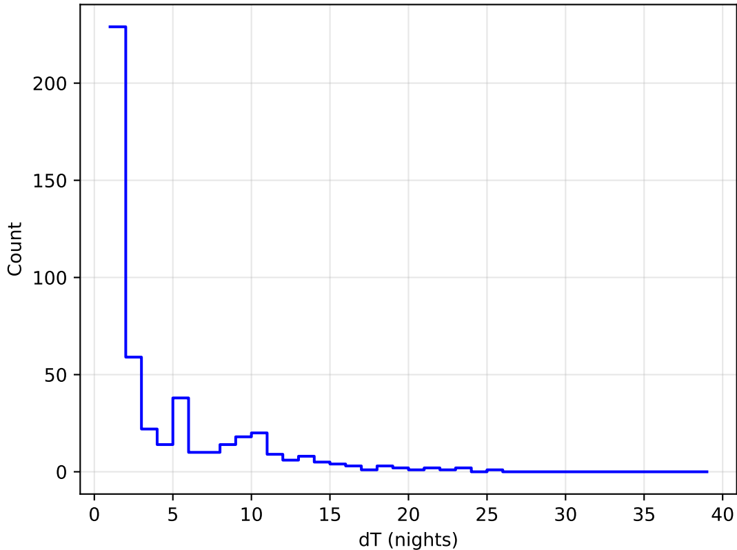
roll_pause_mjdp0_v3.4_10yrs all bands: DD: COSMOS Delta Nights Histogram
