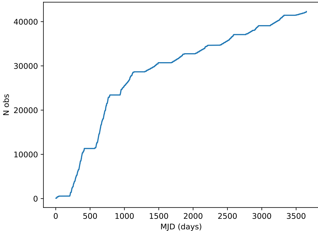
roll_pause_mjdp0_v3.4_10yrs all bands: DD:COSMOS Cumulative NVisits
