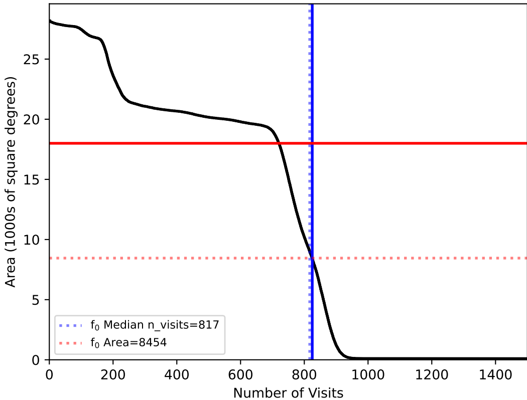
roll_mid3_const_season2v3.3_10yrs : f0
