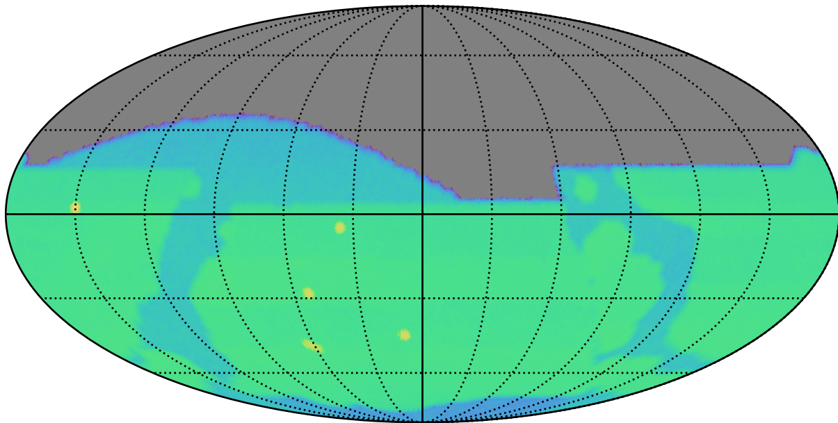
roll_mid3_const_season2v3.3_10yrs r: SurfaceBrightLimit
