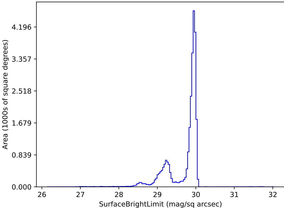
roll_mid3_const_season2v3.3_10yrs i: SurfaceBrightLimit
