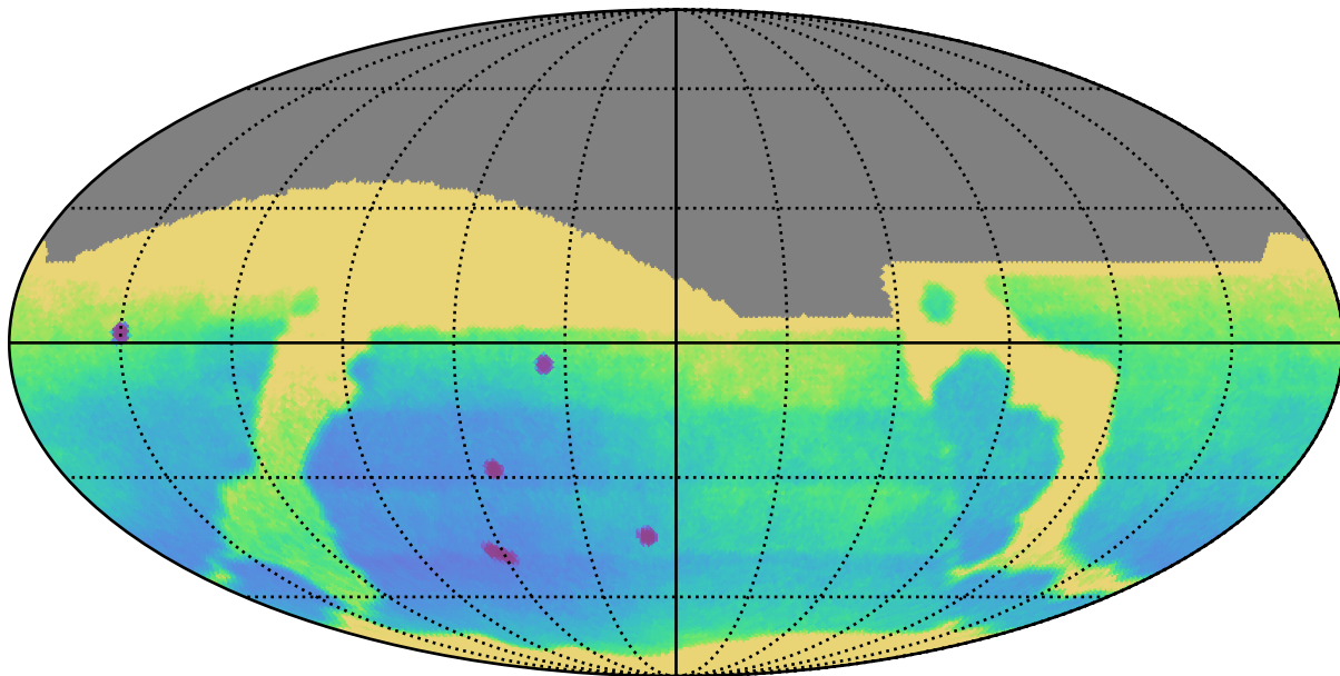
roll_mid3_const_season2v3.3_10yrs : Parallax Uncert @ 24.0
