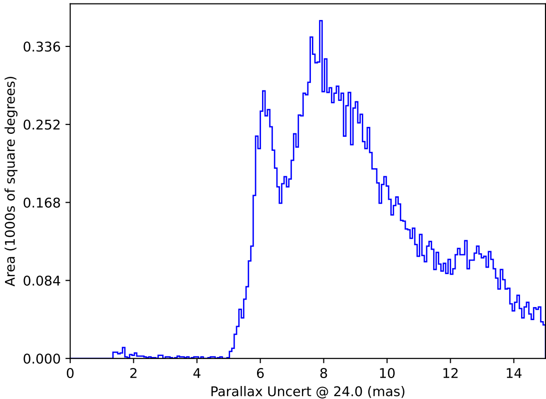
roll_mid3_const_season2v3.3_10yrs : Parallax Uncert @ 24.0
