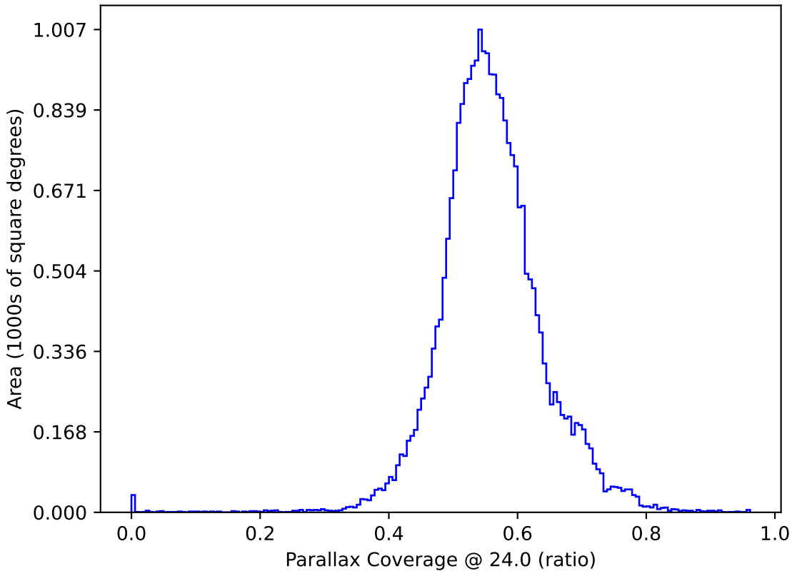
roll_mid3_const_season2v3.3_10yrs : Parallax Coverage @ 24.0
