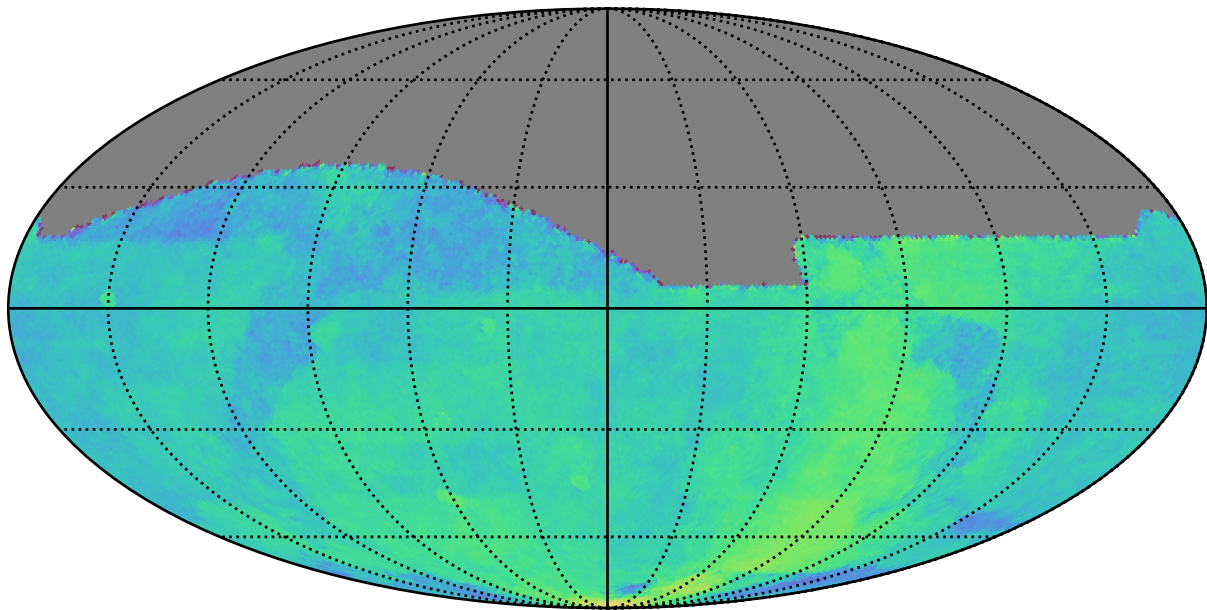
roll_mid3_const_season2v3.3_10yrs : Parallax Coverage @ 22.4
