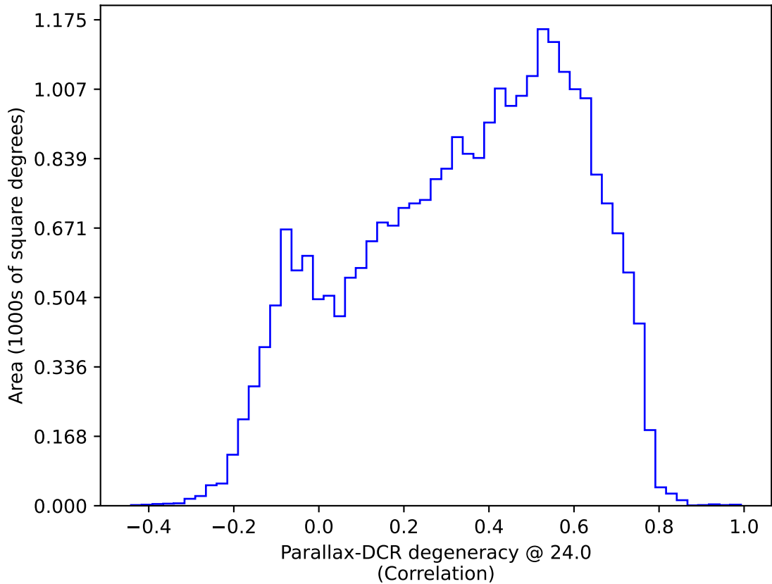
roll_mid3_const_season2v3.3_10yrs : Parallax-DCR degeneracy @ 24.0
