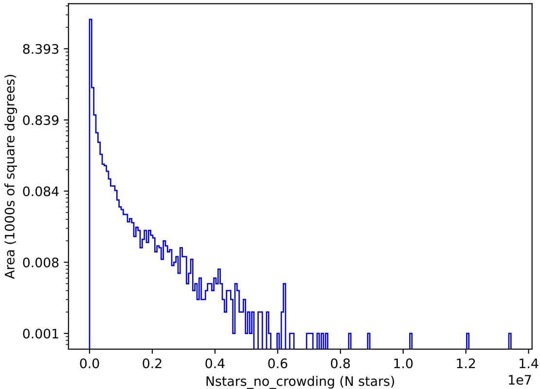
roll_mid3_const_season2v3.3_10yrs g: Nstars_no_crowding
