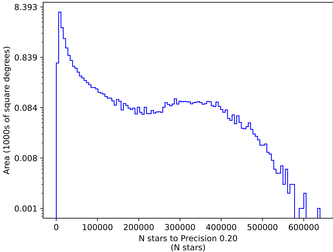
roll_mid3_const_season2v3.3_10yrs y: N stars to Precision 0.20
