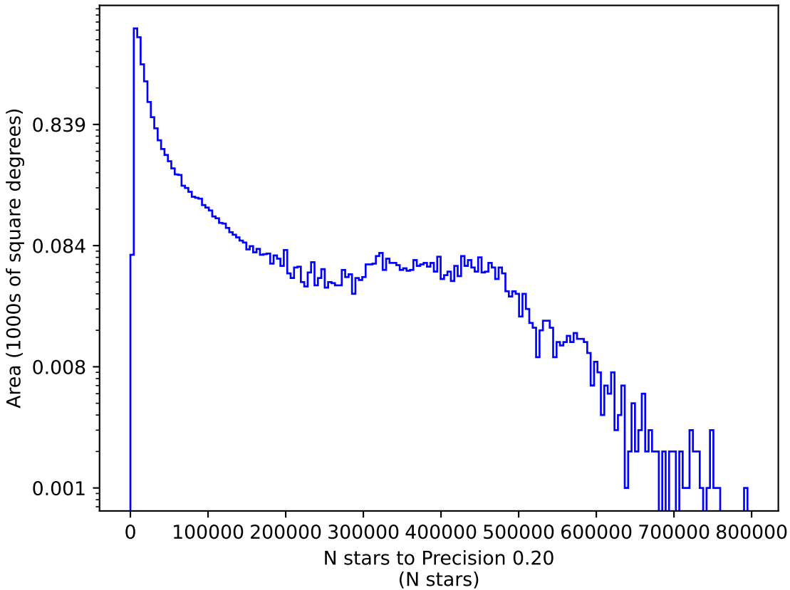
roll_mid3_const_season2v3.3_10yrs r: N stars to Precision 0.20
