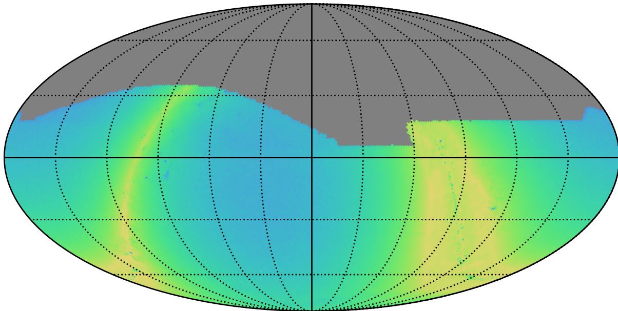
roll_mid3_const_season2v3.3_10yrs i: N stars to Precision 0.20
