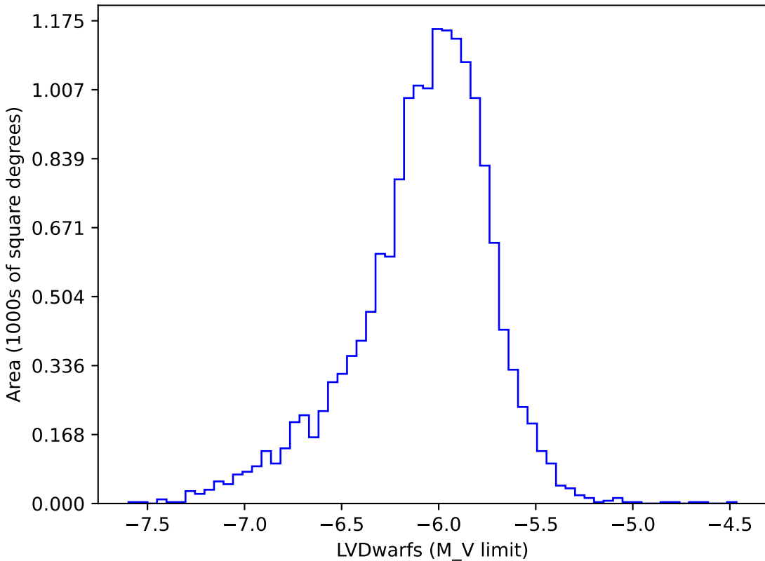
roll_mid3_const_season2v3.3_10yrs gi: LVDwarfs
