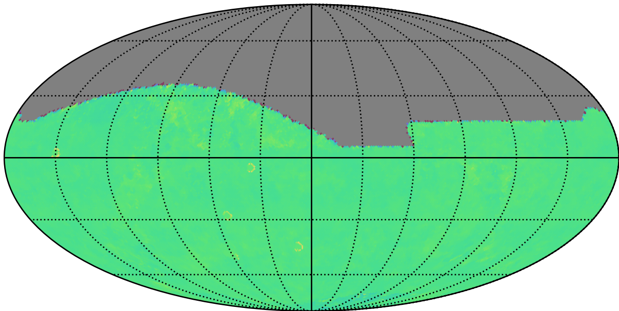
roll_mid3_const_season2v3.3_10yrs z: Kuiper rotTelPos
