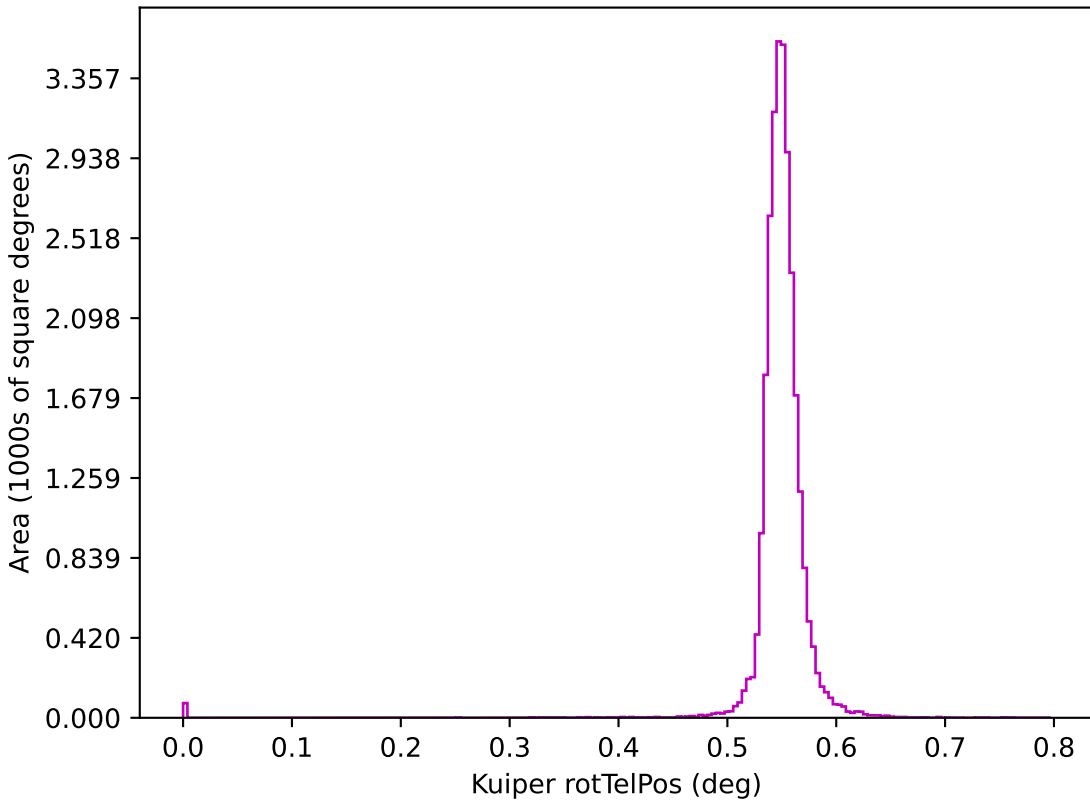
roll_mid3_const_season2v3.3_10yrs z: Kuiper rotTelPos
