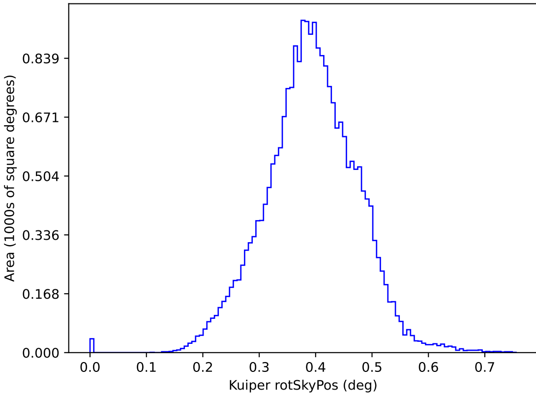
roll_mid3_const_season2v3.3_10yrs y: Kuiper rotSkyPos
