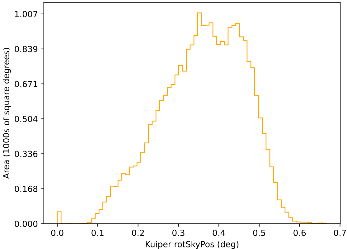
roll_mid3_const_season2v3.3_10yrs r: Kuiper rotSkyPos
