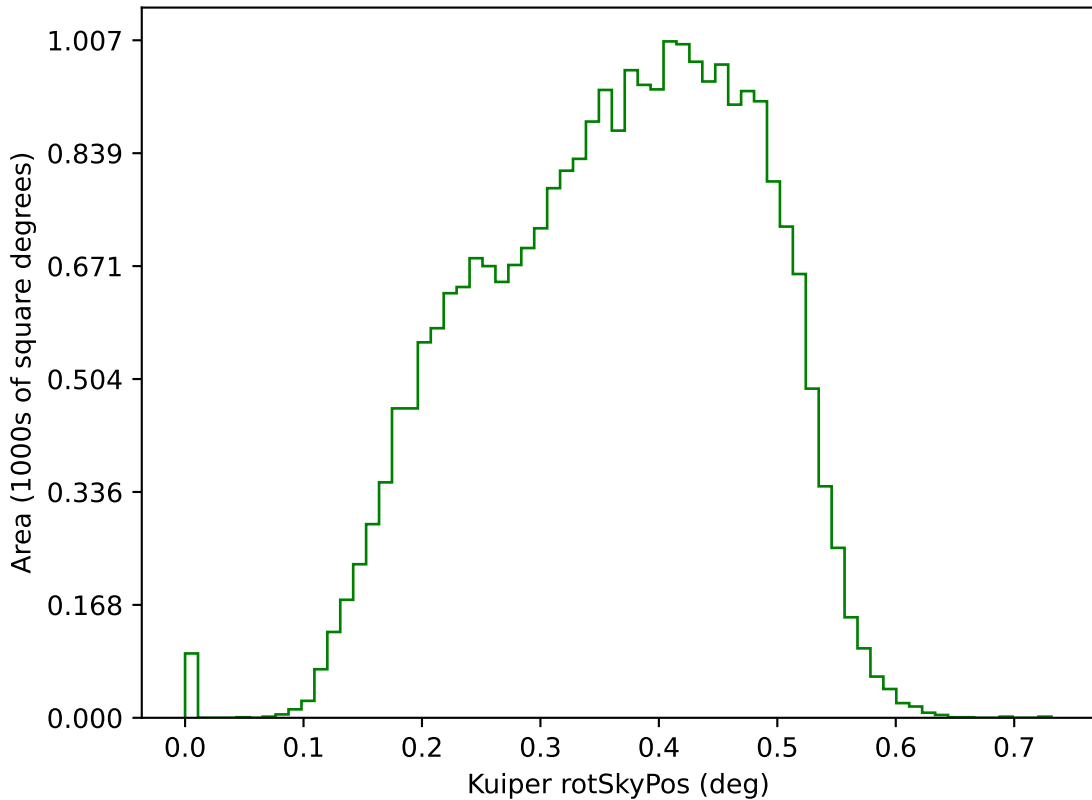
roll_mid3_const_season2v3.3_10yrs g: Kuiper rotSkyPos
