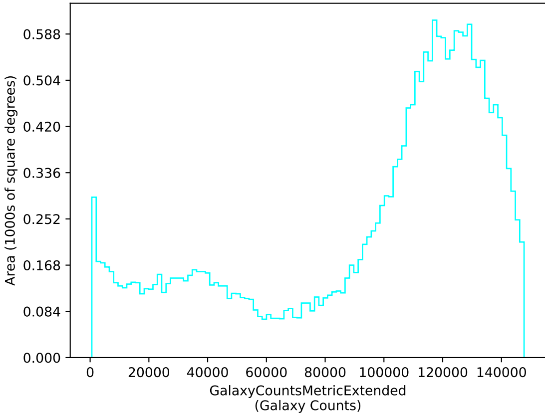
roll_mid3_const_season2v3.3_10yrs u: GalaxyCountsMetricExtended
