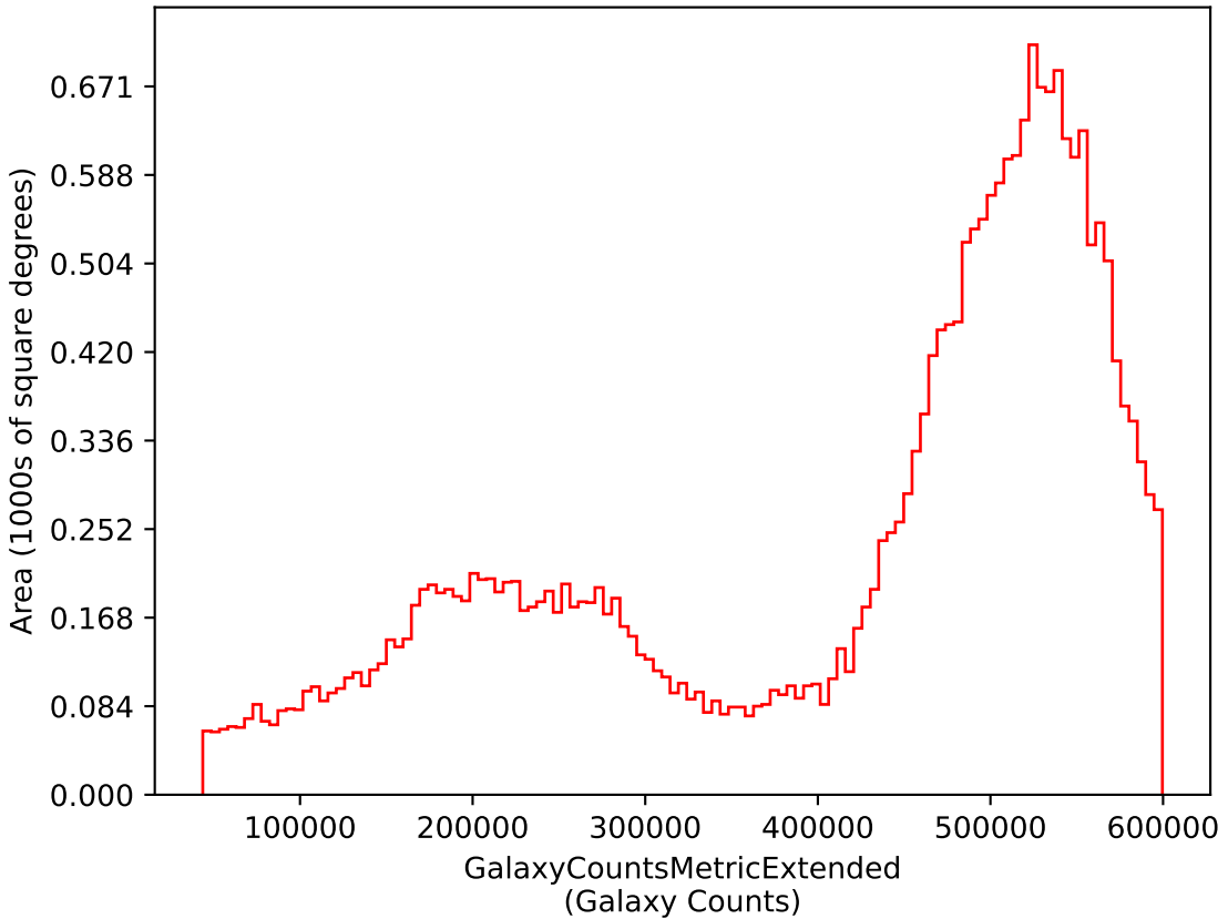
roll_mid3_const_season2v3.3_10yrs i: GalaxyCountsMetricExtended
