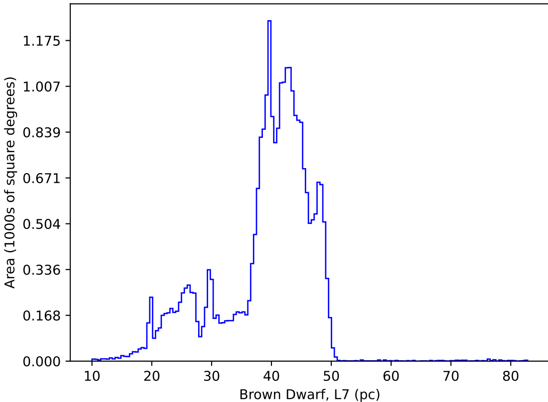
roll_mid3_const_season2v3.3_10yrs : Brown Dwarf, L7
