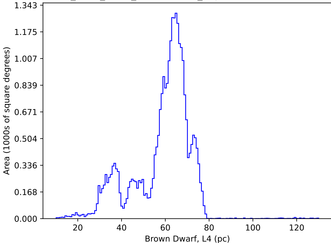
roll_mid3_const_season2v3.3_10yrs : Brown Dwarf, L4
