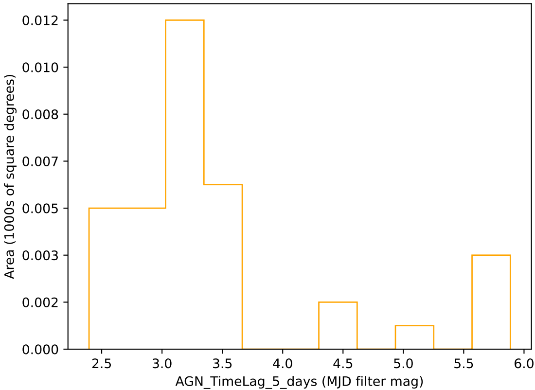
roll_mid3_const_season2v3.3_10yrs r band: AGN_TimeLag_5_days
