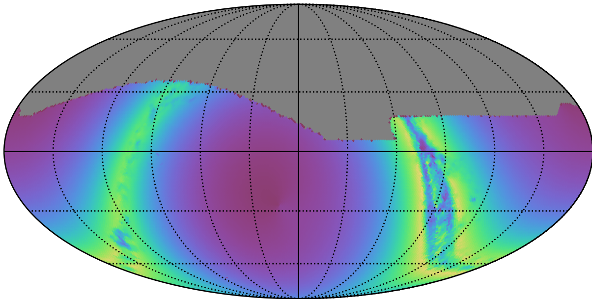
roll_mid2_const_season_v3.3_10yrs : young_stars
