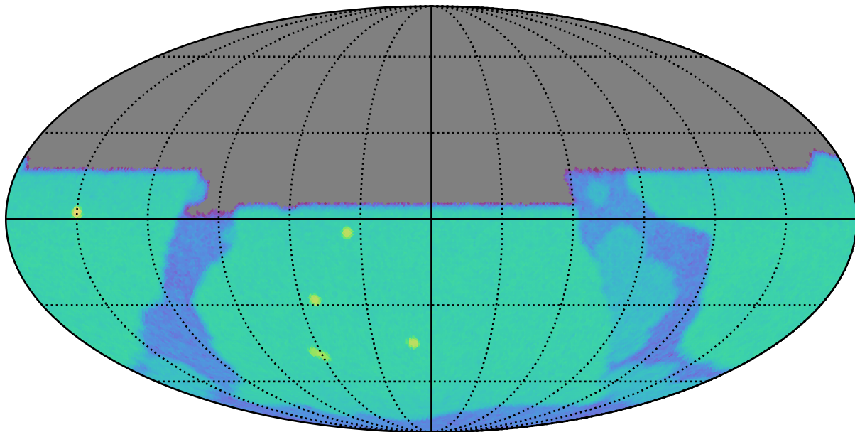
roll_mid2_const_season_v3.3_10yrs u: SurfaceBrightLimit
