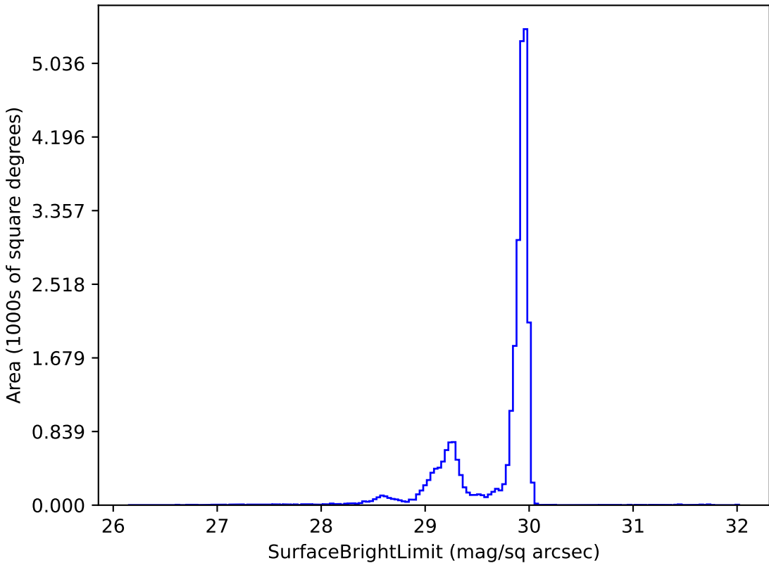
roll_mid2_const_season_v3.3_10yrs i: SurfaceBrightLimit
