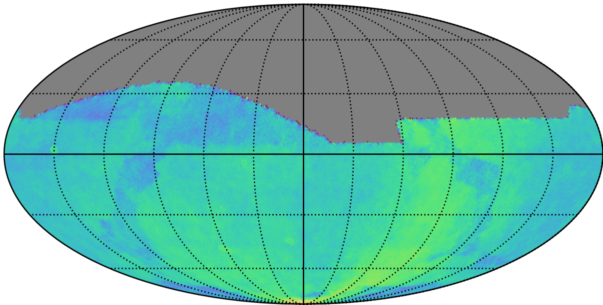
roll_mid2_const_season_v3.3_10yrs : Parallax Coverage @ 22.4
