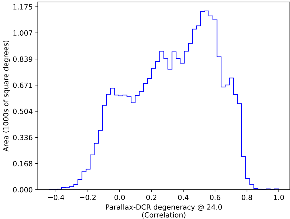
roll_mid2_const_season_v3.3_10yrs : Parallax-DCR degeneracy @ 24.0
