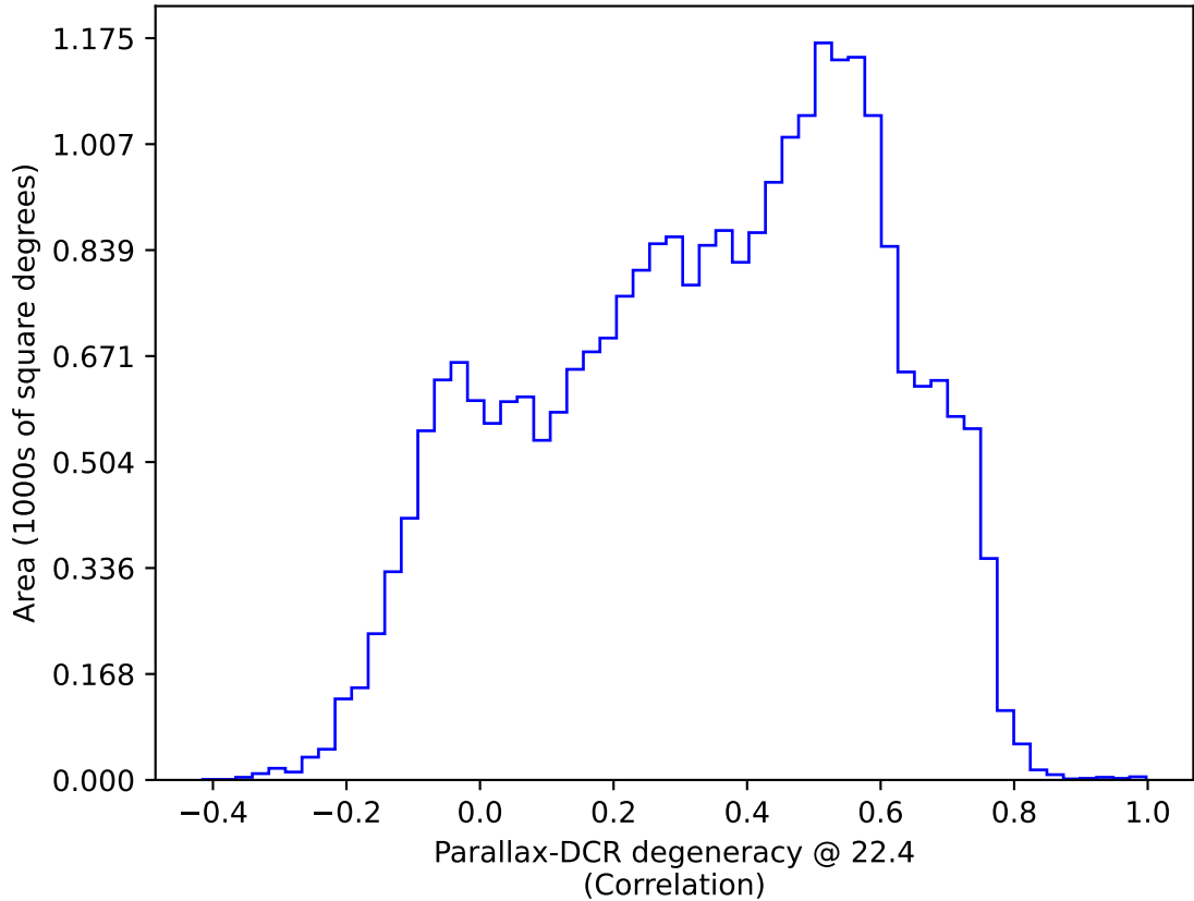
roll_mid2_const_season_v3.3_10yrs : Parallax-DCR degeneracy @ 22.4
