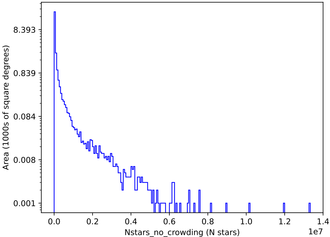
roll_mid2_const_season_v3.3_10yrs g: Nstars_no_crowding
