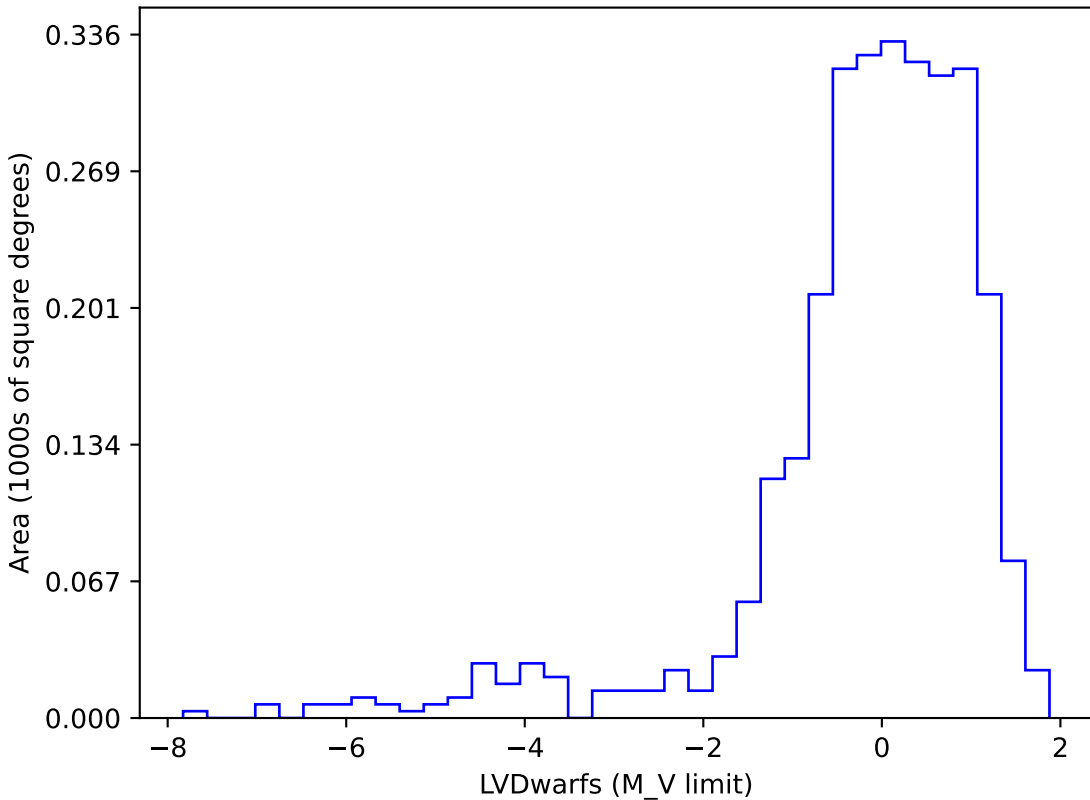
roll_mid2_const_season_v3.3_10yrs gi SCP: LVDwarfs
