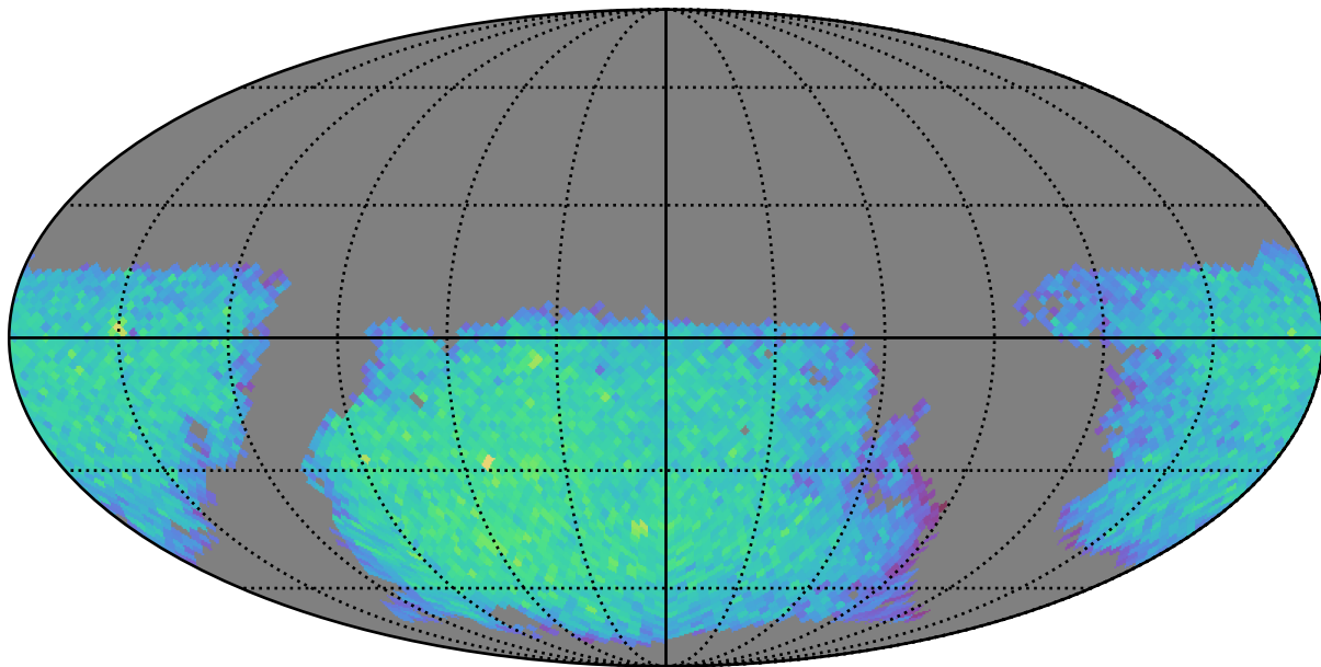
roll_mid2_const_season_v3.3_10yrs gi: LVDwarfs
