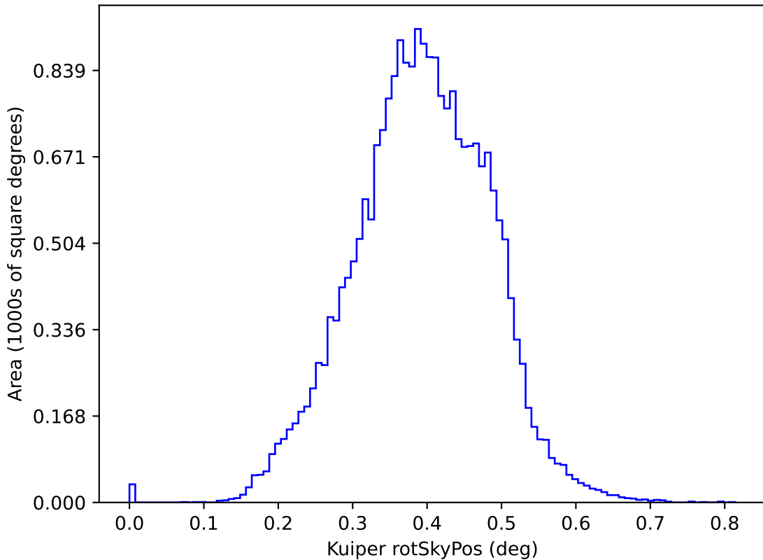
roll_mid2_const_season_v3.3_10yrs y: Kuiper rotSkyPos
