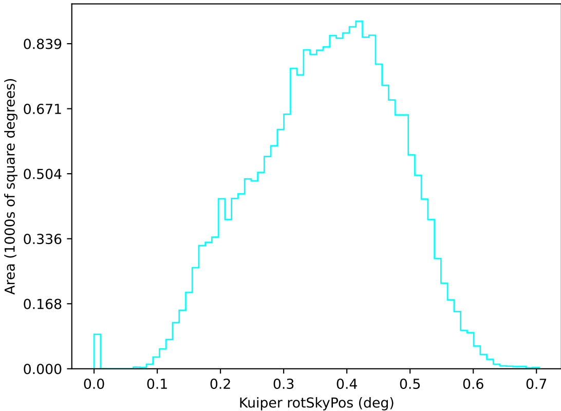
roll_mid2_const_season_v3.3_10yrs u: Kuiper rotSkyPos
