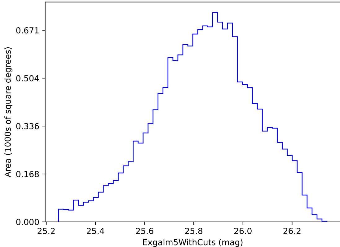
roll_mid2_const_season_v3.3_10yrs i band non-DD year 3: ExgalM5WithCuts
