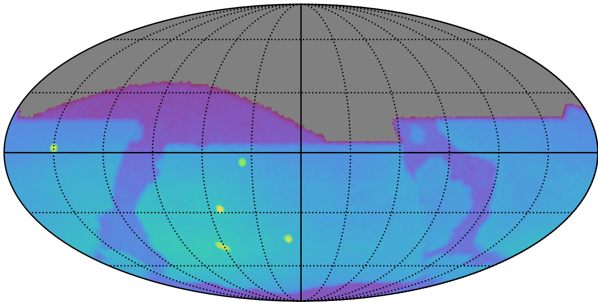
roll_mid2_const_season_v3.3_10yrs : Brown Dwarf, L4
