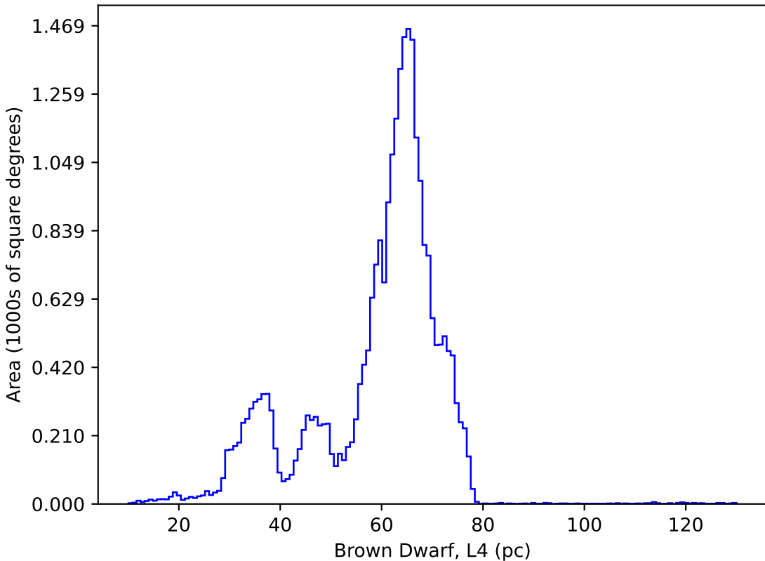
roll_mid2_const_season_v3.3_10yrs : Brown Dwarf, L4
