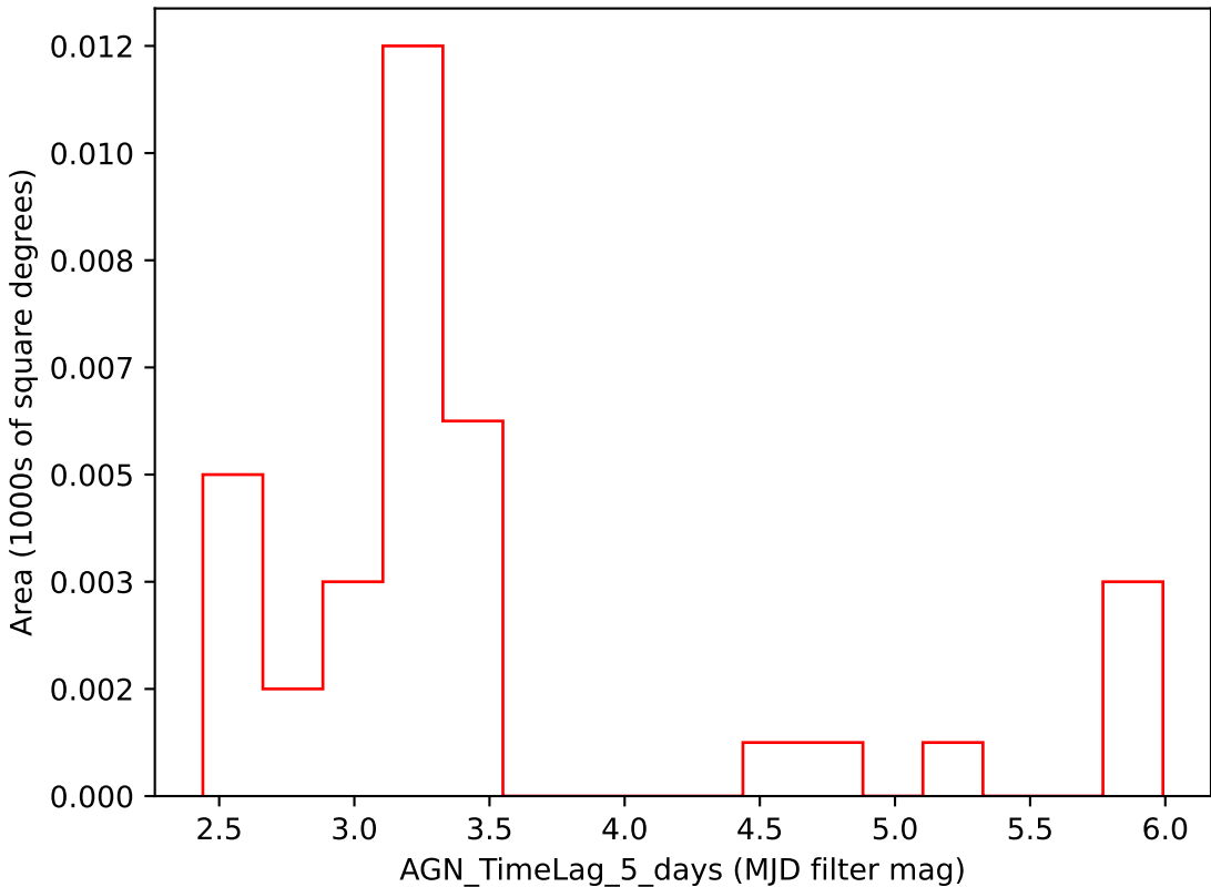
roll_mid2_const_season_v3.3_10yrs i band: AGN_TimeLag_5_days
