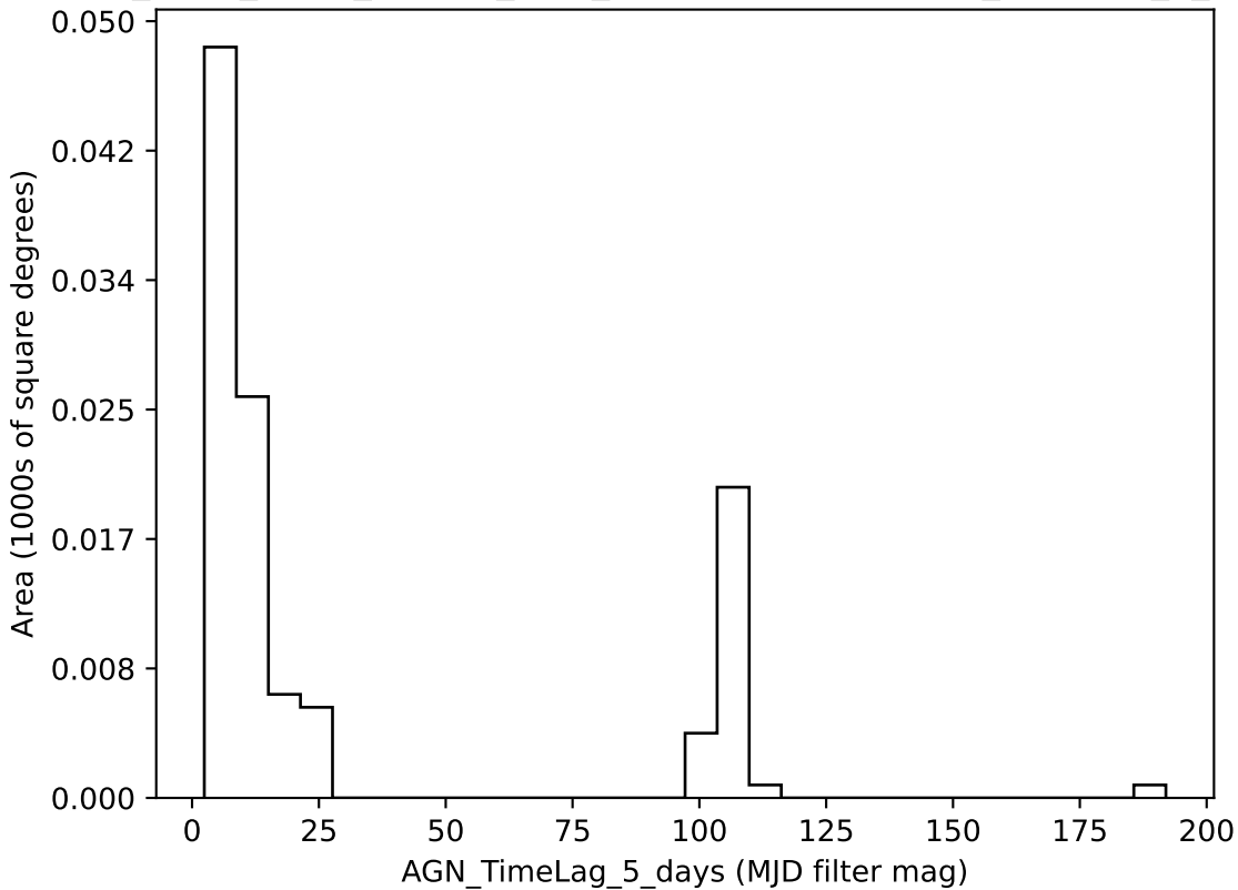
roll_mid2_const_season_v3.3_10yrs all bands: AGN_TimeLag_5_days
